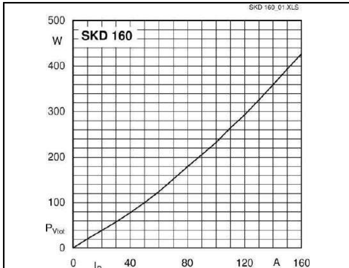
Fig. 3L Power dissipation vs. output current
