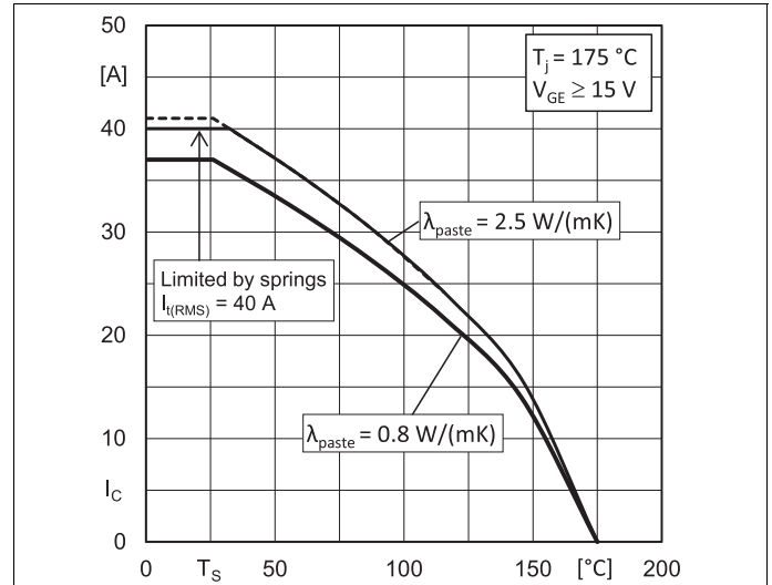
Fig. 2: Typ. rated current vs. temperature I_C = f(T_j)
