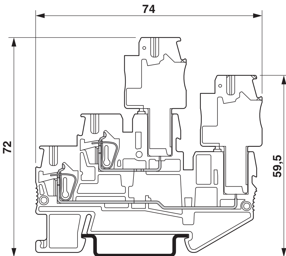
Dimensional drawing
