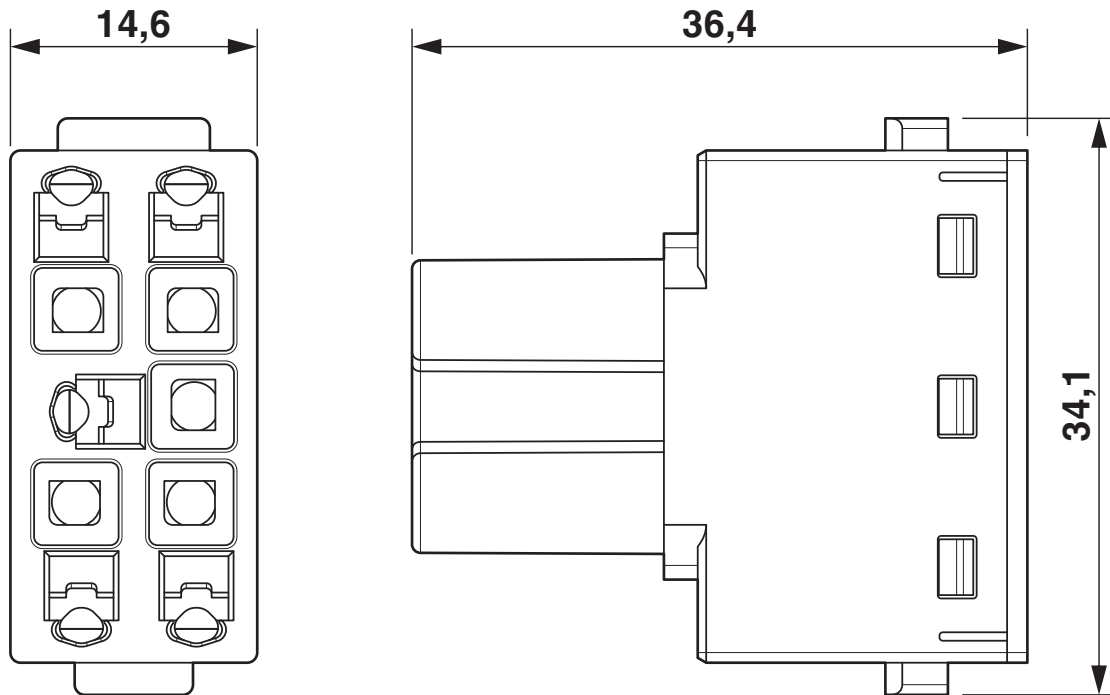
Dimensional drawing
