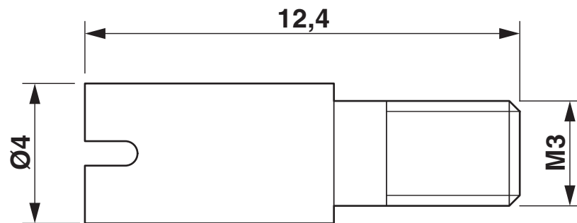
Dimensional drawing
