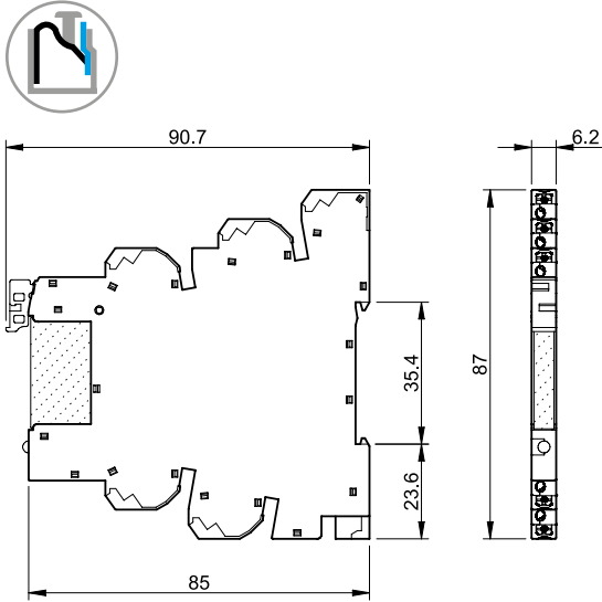
39.00/39.01 39.50/39.51 Push-in terminal
