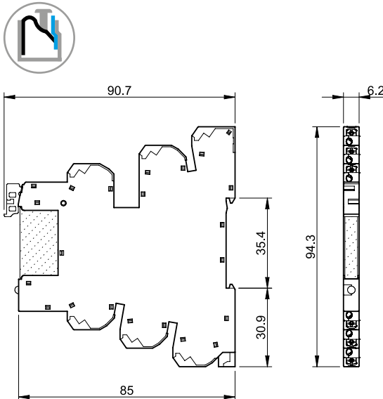
39.70 39.71 Push-in terminal
