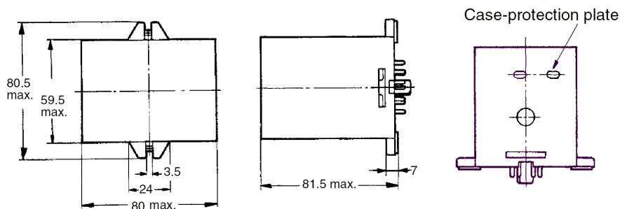
Outline drawing
