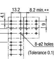
Terminal Arrangement
