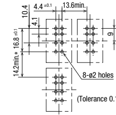
Terminal Arrangement
