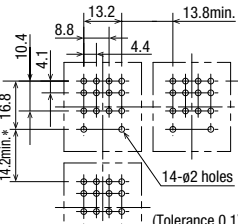
Terminal Arrangement
