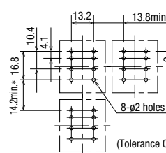
Terminal Arrangement
