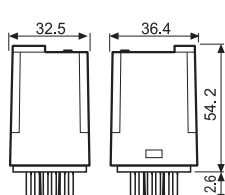
Type 60.13/60.13 - 52xx
