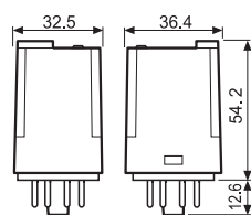
Type 60.12/60.12 - 52xx
