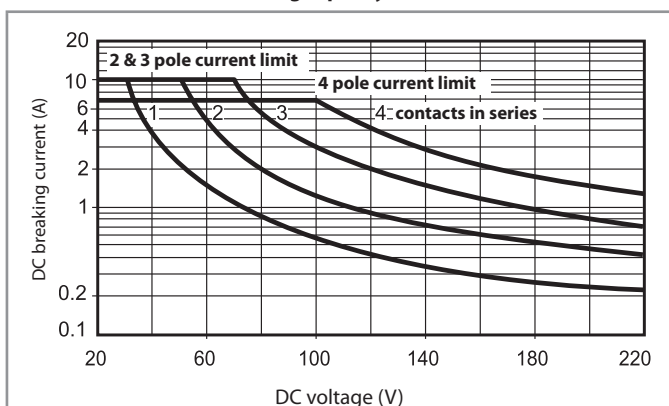
H 55 - Maximum DC1 breaking capacity
