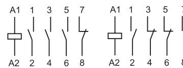
3 NO + 1 NC (4710)
